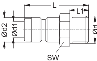
Plug with thread Nippel Aussengewinde
